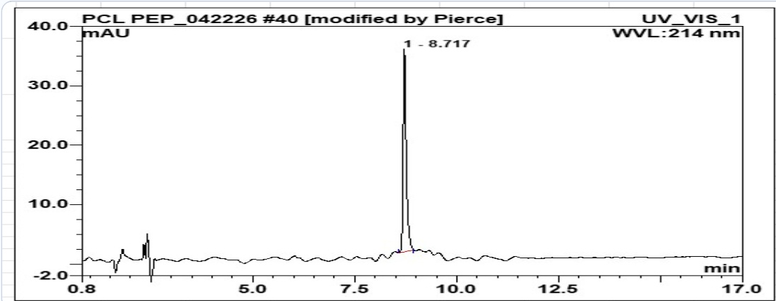
HPLC Chromatogram (Retention Time: 8.717 min)
