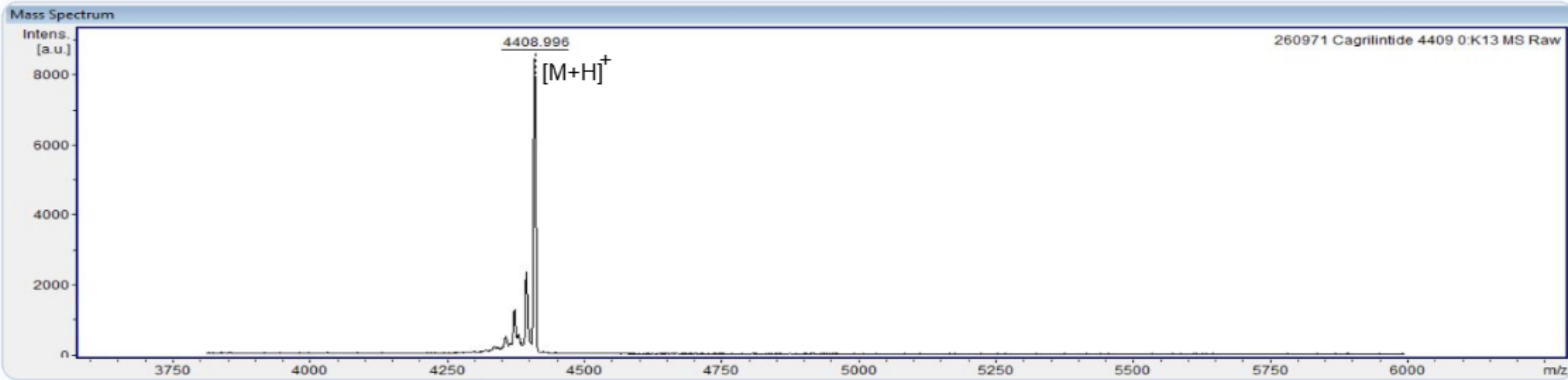
Mass Spectrum (MALDI-MS)
